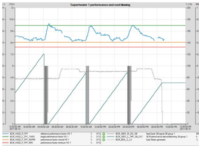
Fouling trend
